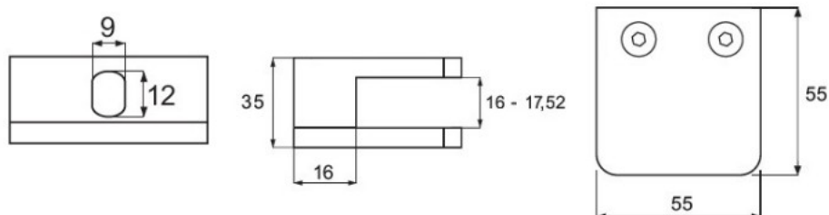
Cushions for stainless steel model
